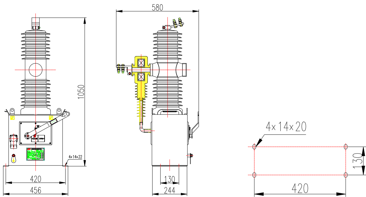
Mounting Dimension of CB
